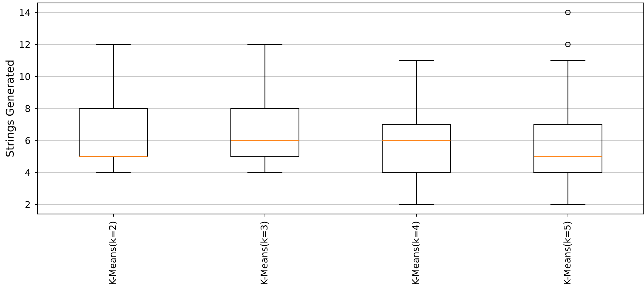
YARA Rules Strings Generated Distribution (Cluster44_Size5 dataset)
